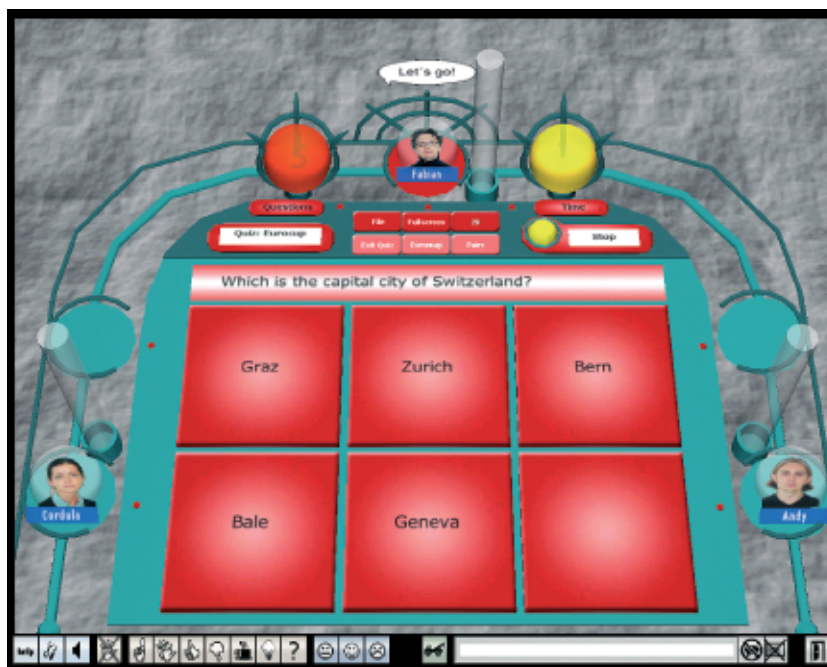
Figure 6: YoungNet Quiz
