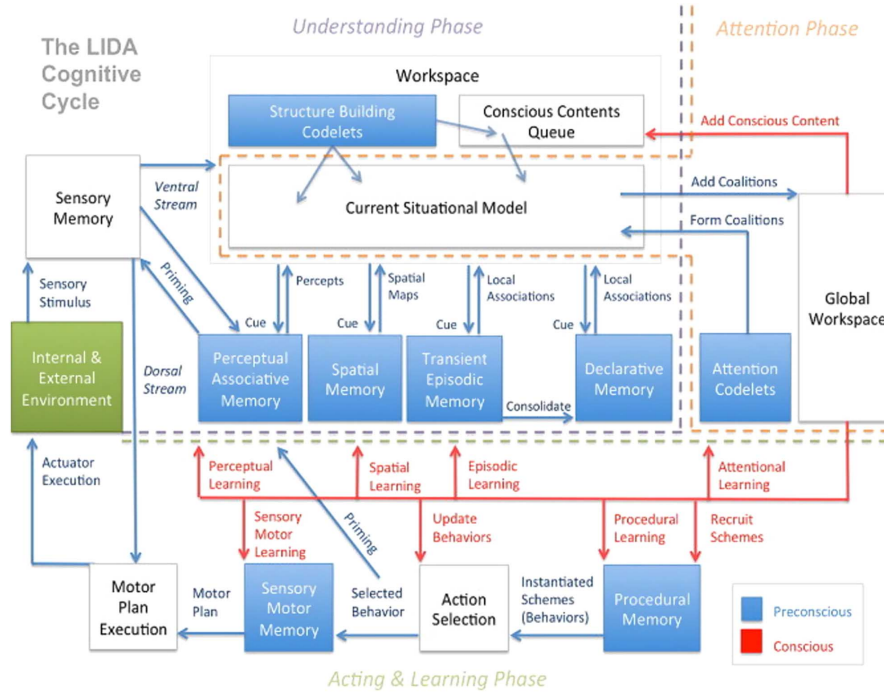
Fig. 1 LIDA cognitive cycle diagram.
