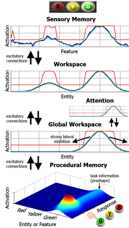
Fig. 3 Dynamical systems (DFT) based implementation of the LIDA cognitive cycle in a reaction time experiment. The blue, thick lines / blue surface represent dynamic neural fields. Red, thin lines show the field output, after the application of a sigmoidal threshold function to ensure that only sufficiently activated field sites contribute to the interaction [122]. In this simplified example, yellow and green glowing lights are perceived and represented (only one feature layer is shown, but any number could be combined in workspace representations). The activation peak representing the green light enters the Global workspace, due to the Attention field amplifying its peak (but not the peak associated with the yellow light), and elevates the preshaped procedural memory field above threshold, causing an action to be taken and the button to be pressed (preshaping can ensure that from all applicable actions based on current percepts, only the task-relevant one reaches the threshold, and has been argued to be neurally plausible [129]).
