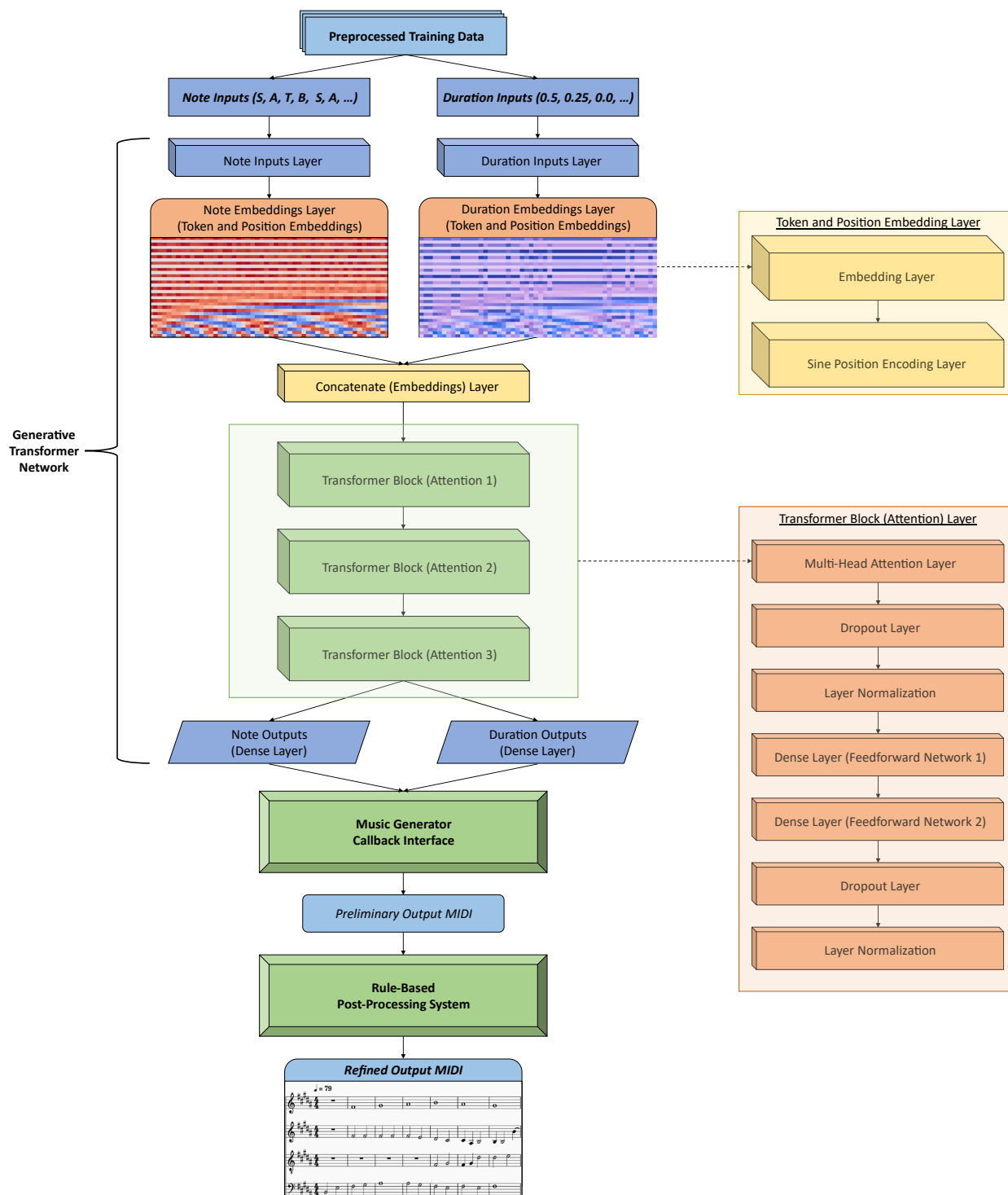
Figure 3.1: Choral-GTN System Architecture Diagram
