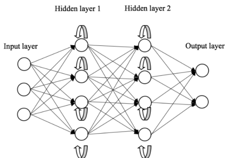
Figure 2.6: A simple Recurrent Neural Network architecture (ODSC Community, 2020)
