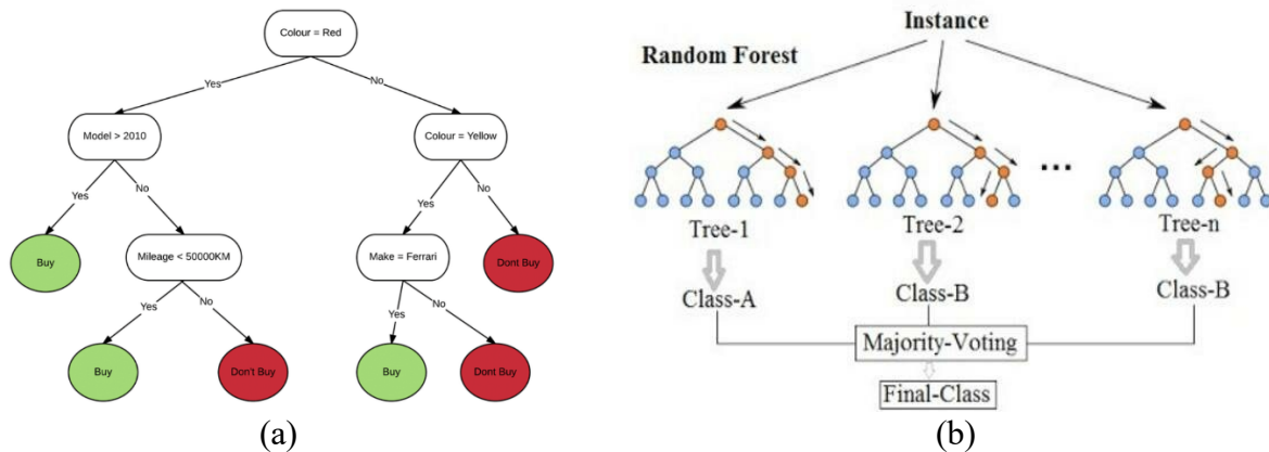
Figure 2.1: Basic decision tree model (a; Kumar, 2022), a random forest (b)
