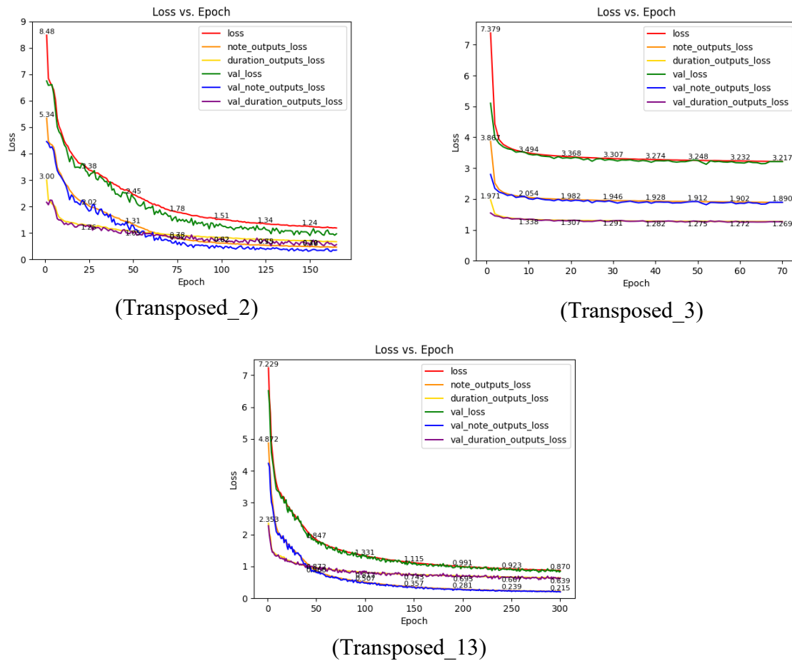
Figure 5.1: Choral-GTN training history plots
