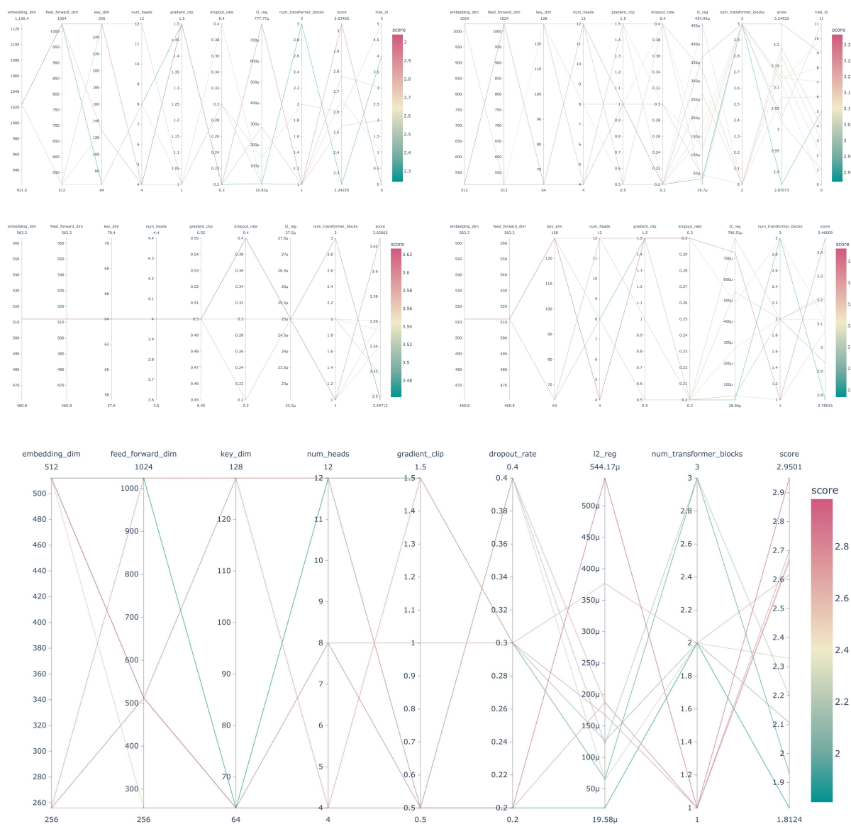
Figure 4.2: Sample parallel coordinates plots from the hyperparameter search trials
