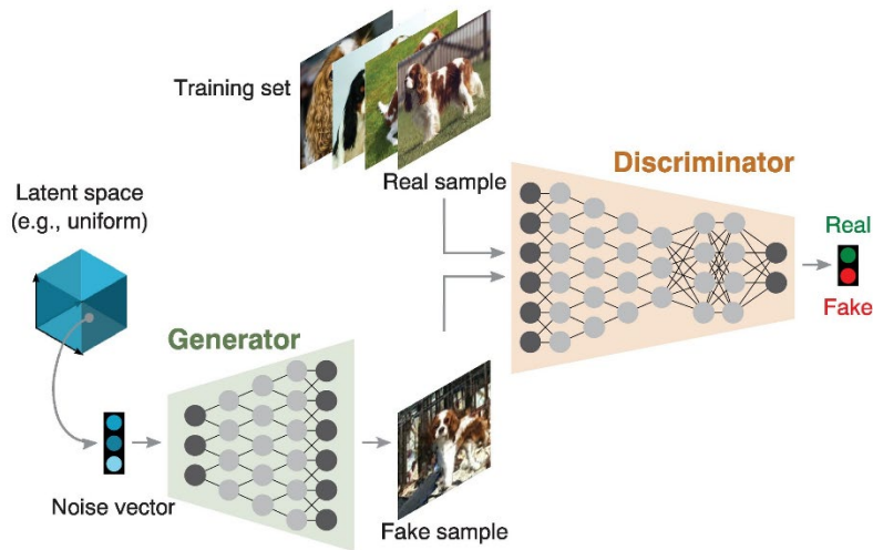
Figure 2.5: A typical GAN architecture (Goetschalckx et al., 2021)
