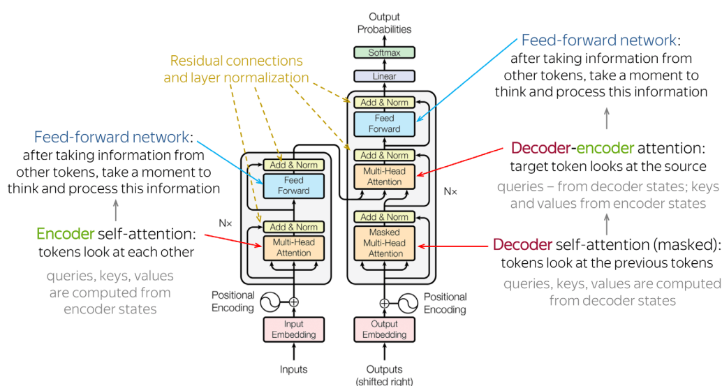
Figure 2.8: Transformer architecture (Voita, 2023)
