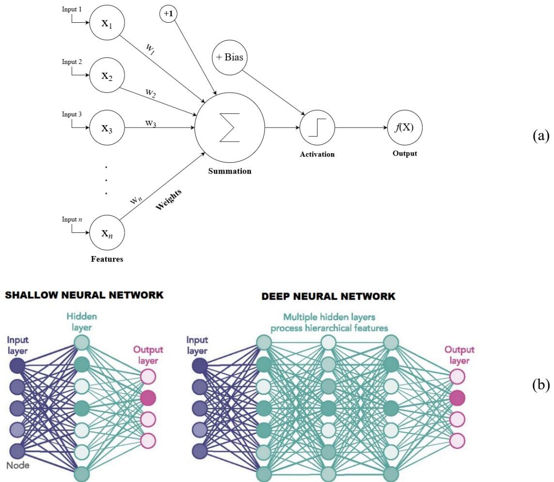
Figure 2.3: A Perceptron (a; Szelogowski, 2022), shallow vs. deep NNs (b; Waldrop, 2019)
