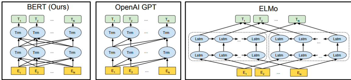
Figure 2.9: BERT, GPT, and ELMo architectures (Lei et al., 2022)
