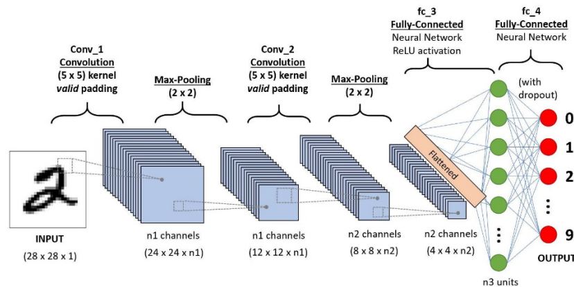
Figure 2.4: A simple Convolutional Neural Network architecture (Suha, 2018)
