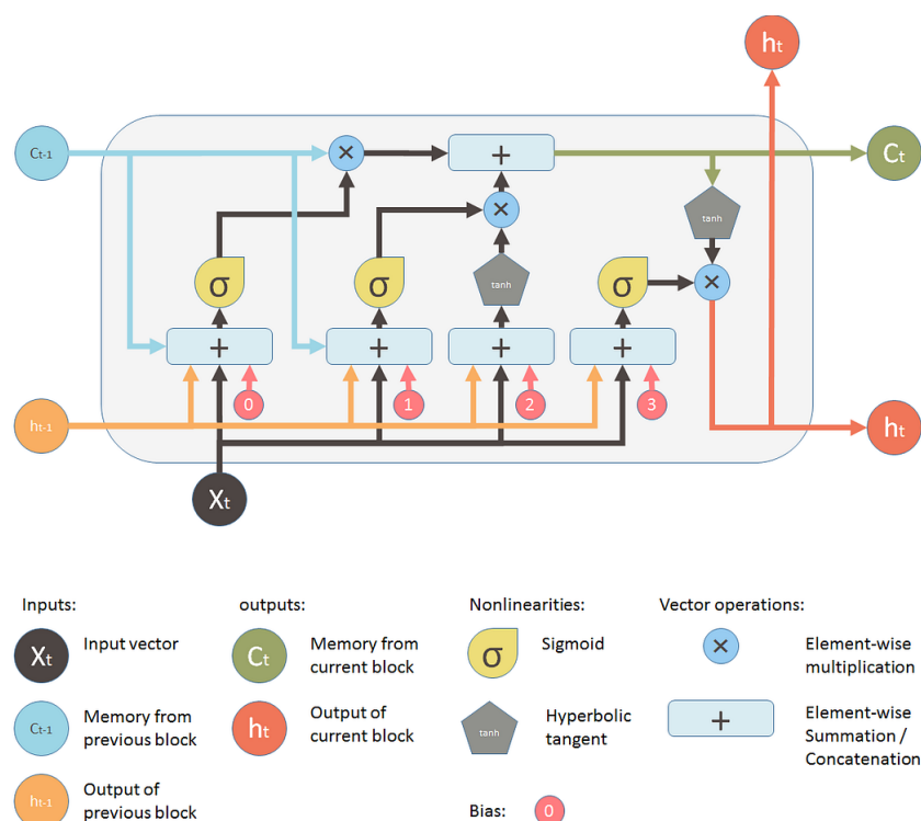
Figure 2.7: Complete LSTM unit (Choubey, 2020)
